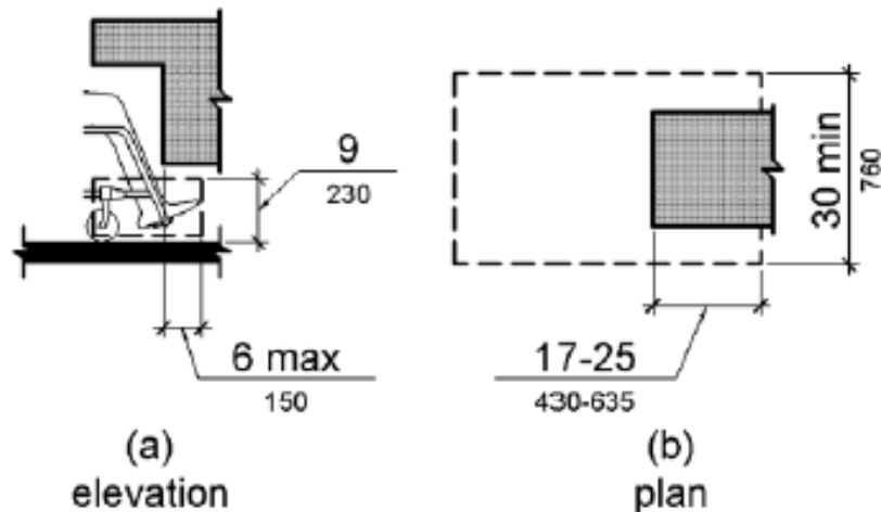
Figure 306.2 Toe Clearance
